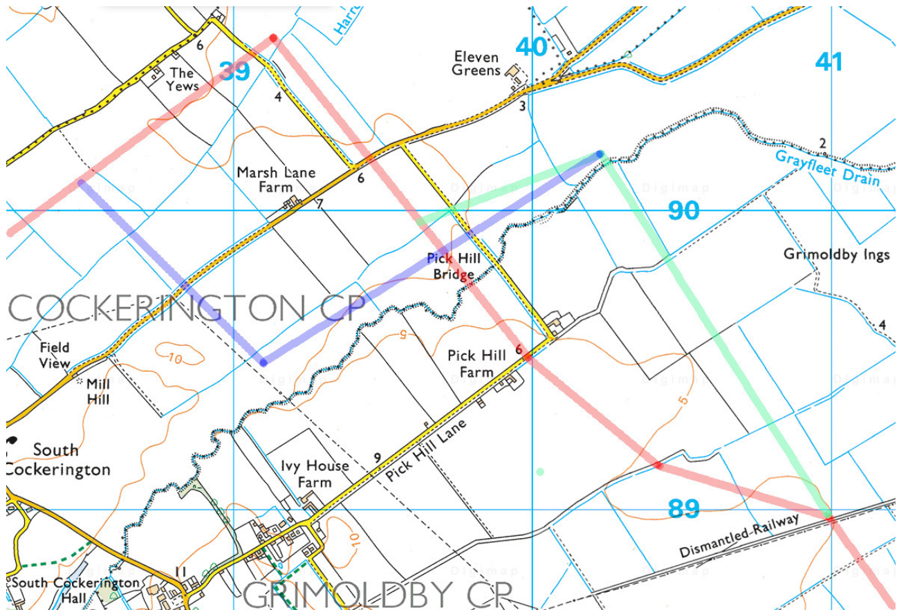
Fig. 2 Alternative 'Safe' Routes (avoiding placing residential properties in severe hazard zones)
